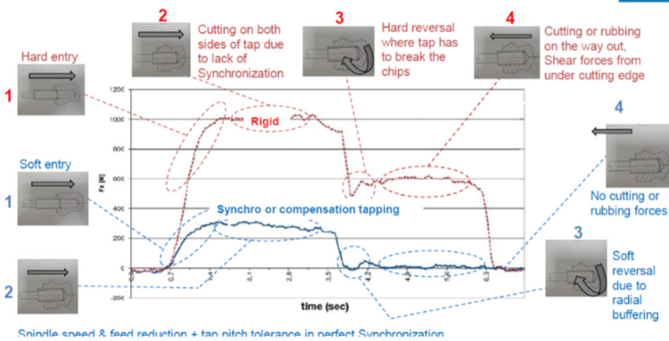
Tapping cycle comparing Rigid Tapping against Synchronized tapping:
